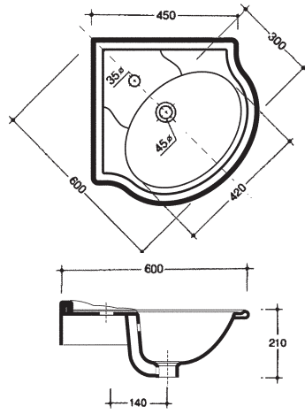
30353 Lavabo angolo Corner washbasin Lavabo angular
